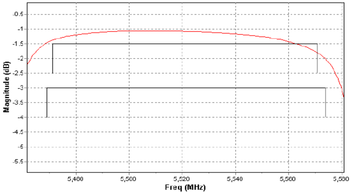
Insertion Loss Simulation Result: Shows that 1.5 dB can be reached @ 5521 MHz
