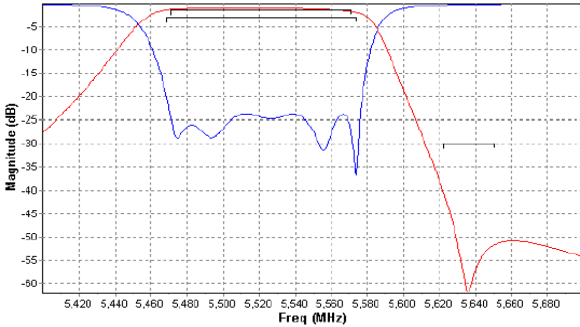
Rejection Performance Simulation Curve
