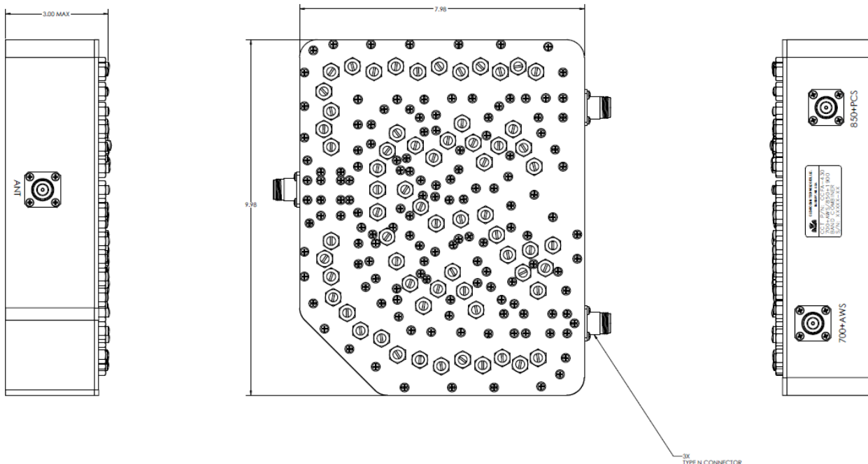
OUTLINE DRAWING
