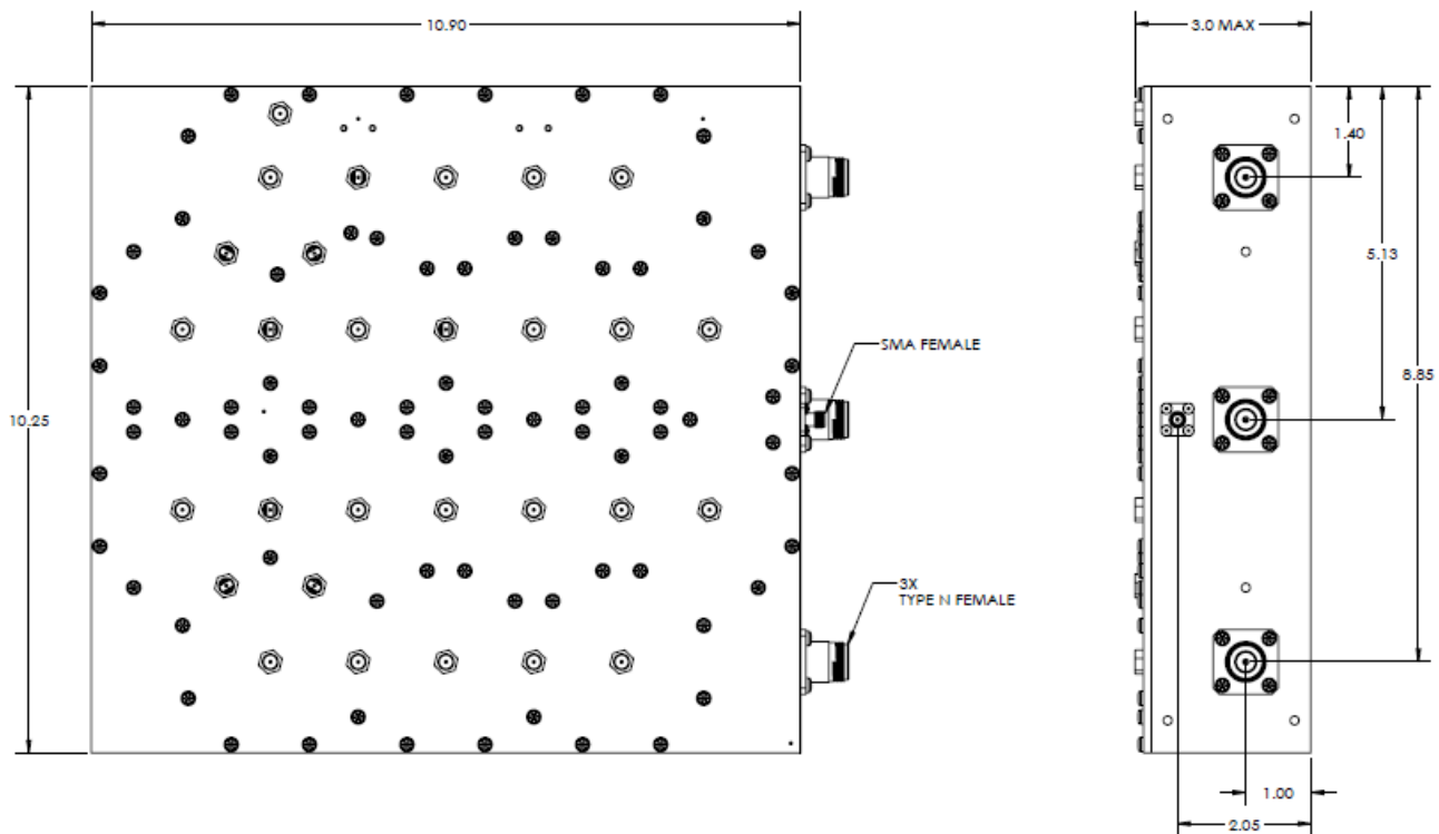
OUTLINE DRAWING
