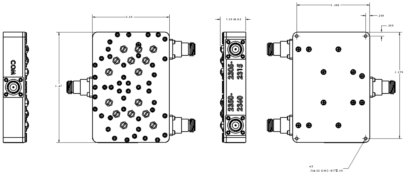
OUTLINE DRAWING
