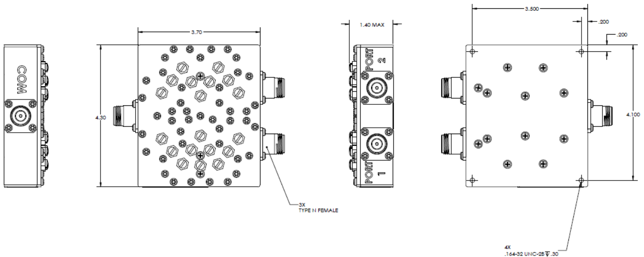
OUTLINE DRAWING
