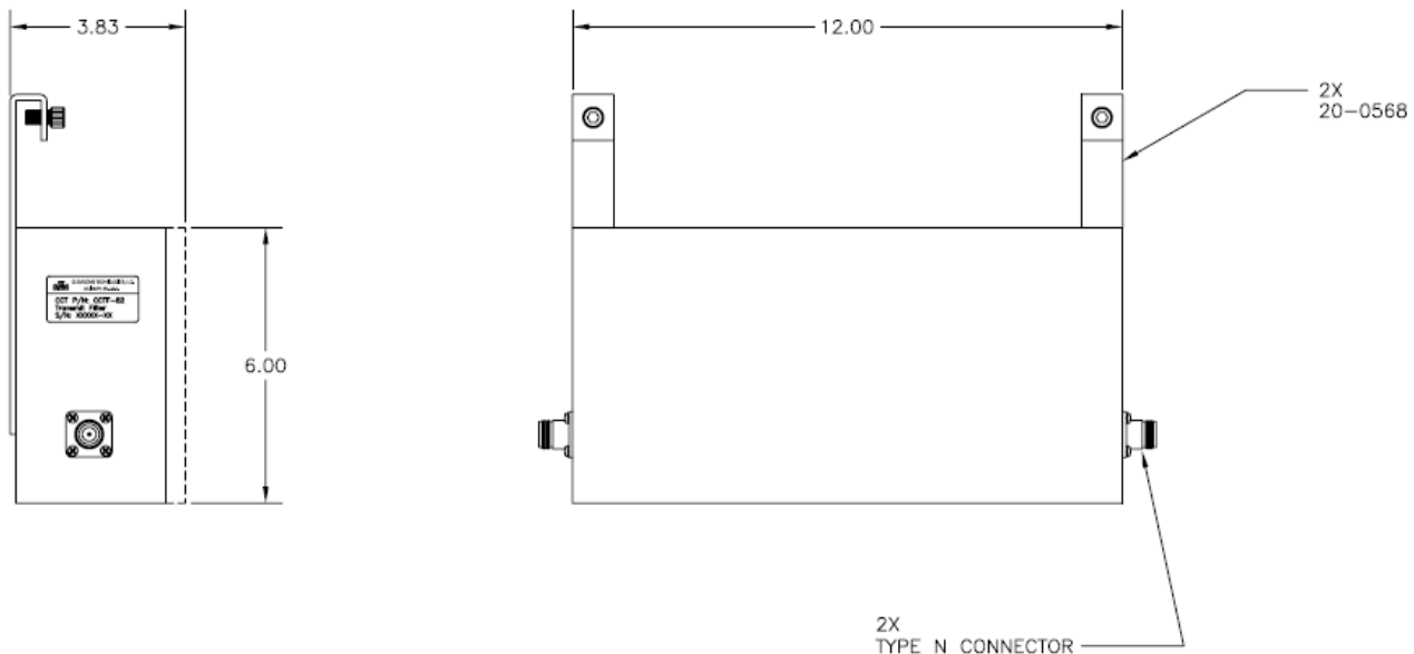
OUTLINE DRAWING
