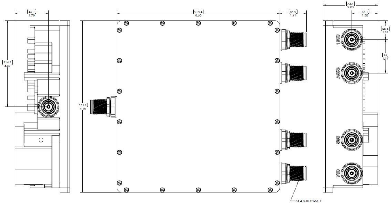
OUTLINE DRAWING
