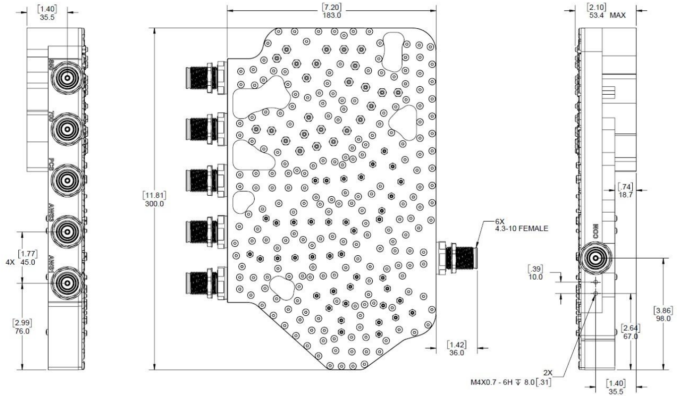
OUTLINE DRAWING
