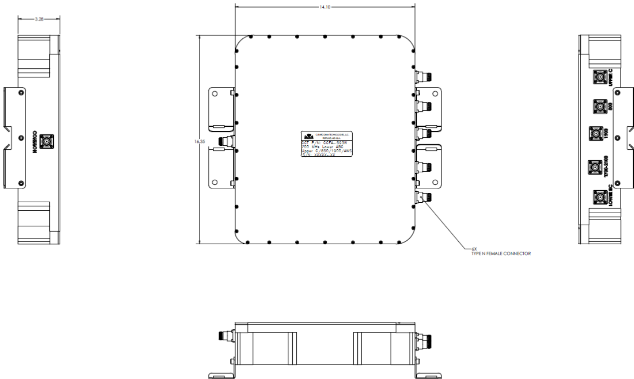
OUTLINE DRAWING
